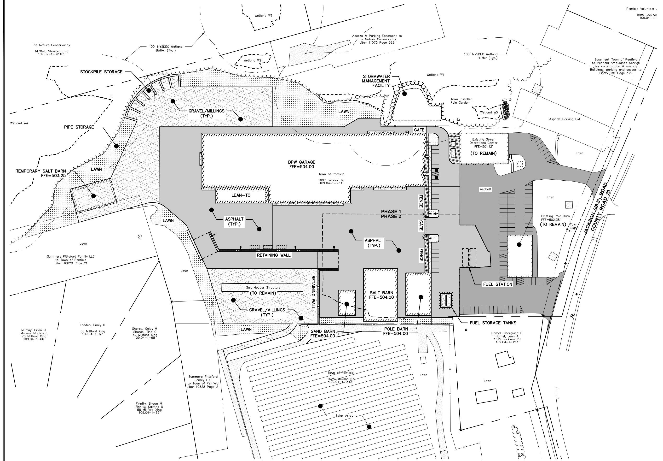
PROPOSED OVERALL SITE PLAN - PHASE 2
