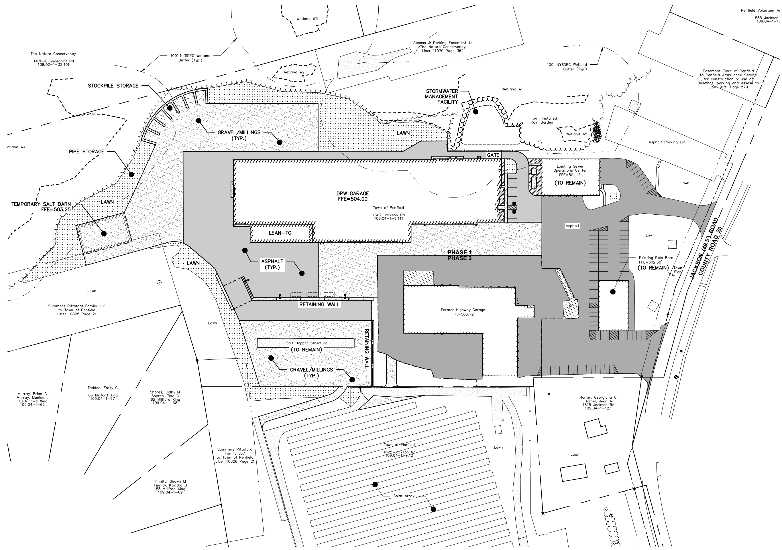
PROPOSED OVERALL SITE PLAN - PHASE 1
